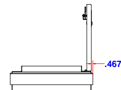
End view showing hinge offset requirements
