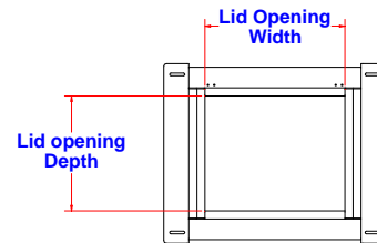
Top view showing door opening requirements
