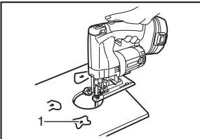
1. Starting hole
