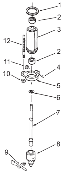
FIGURE 3 QUILL ASSEMBLY
