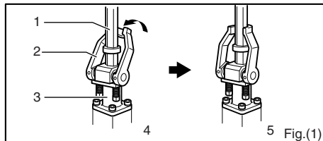
1. Bit 2. Tool retainer 3. Tool holder 4. When the bit is inserted 5. When the bit is retained
